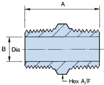
Hexagon Nipple
